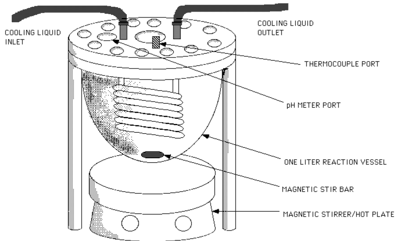
Figure 1. Reaction Vessel
